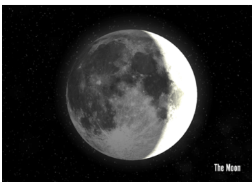
The Moon
