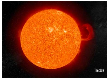
The Sun
